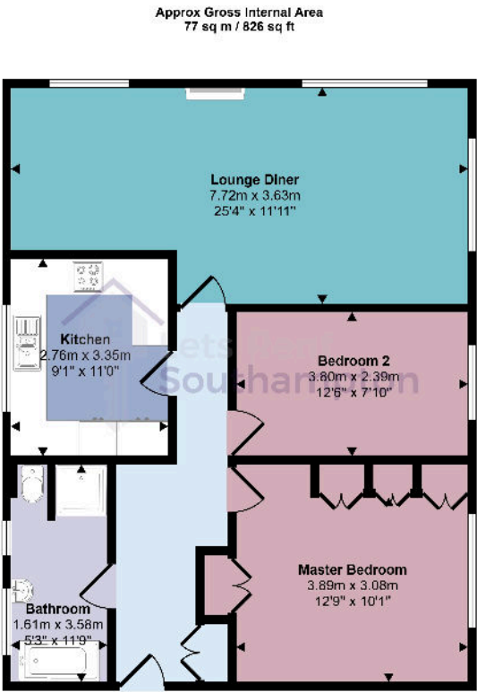
Floorplan
